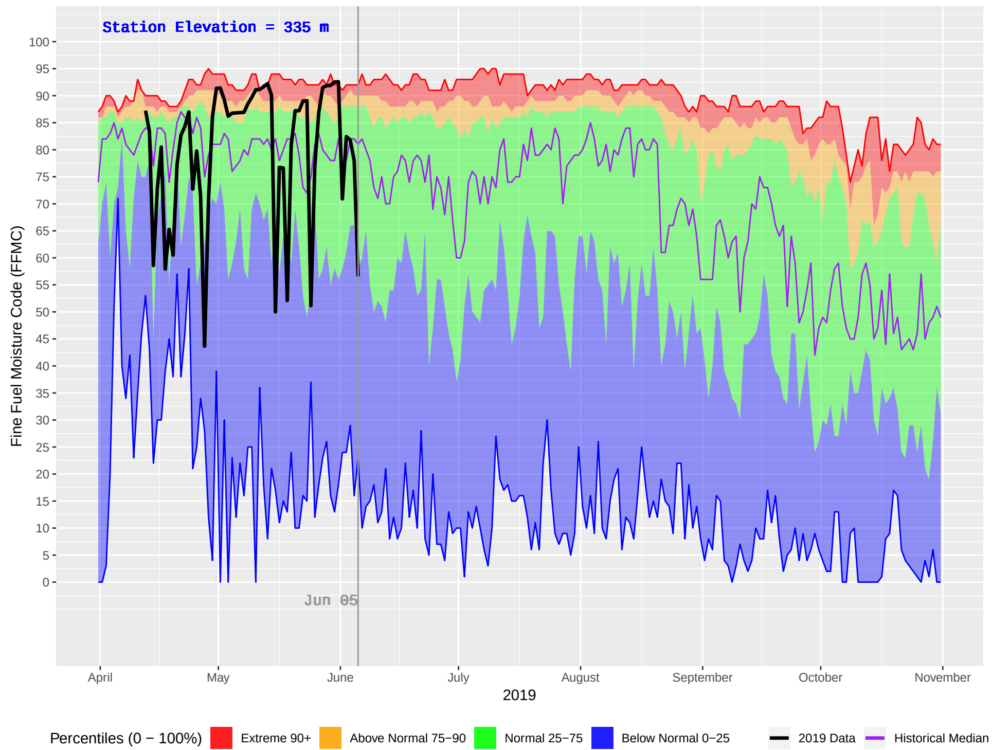
KISPIOX HUB (428) : Historical (1970–2018) and Current (2019) Daily Fine Fuel Moisture Code (FFMC)
