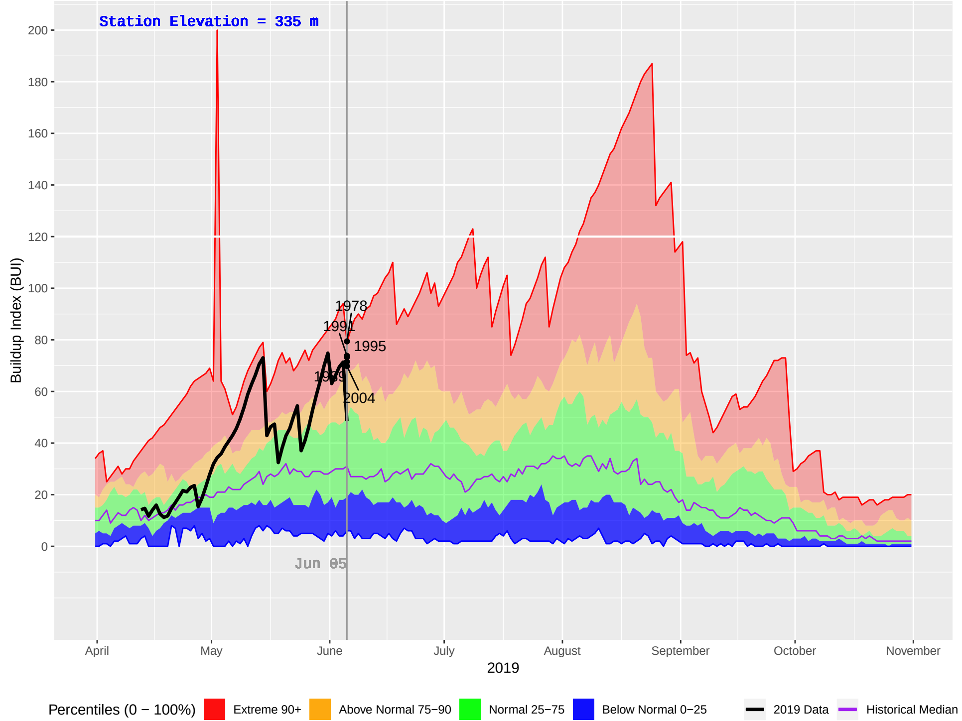
KISPIOX HUB (428) : Historical (1970–2018), Current (2019) Daily Buildup Index (BUI)
