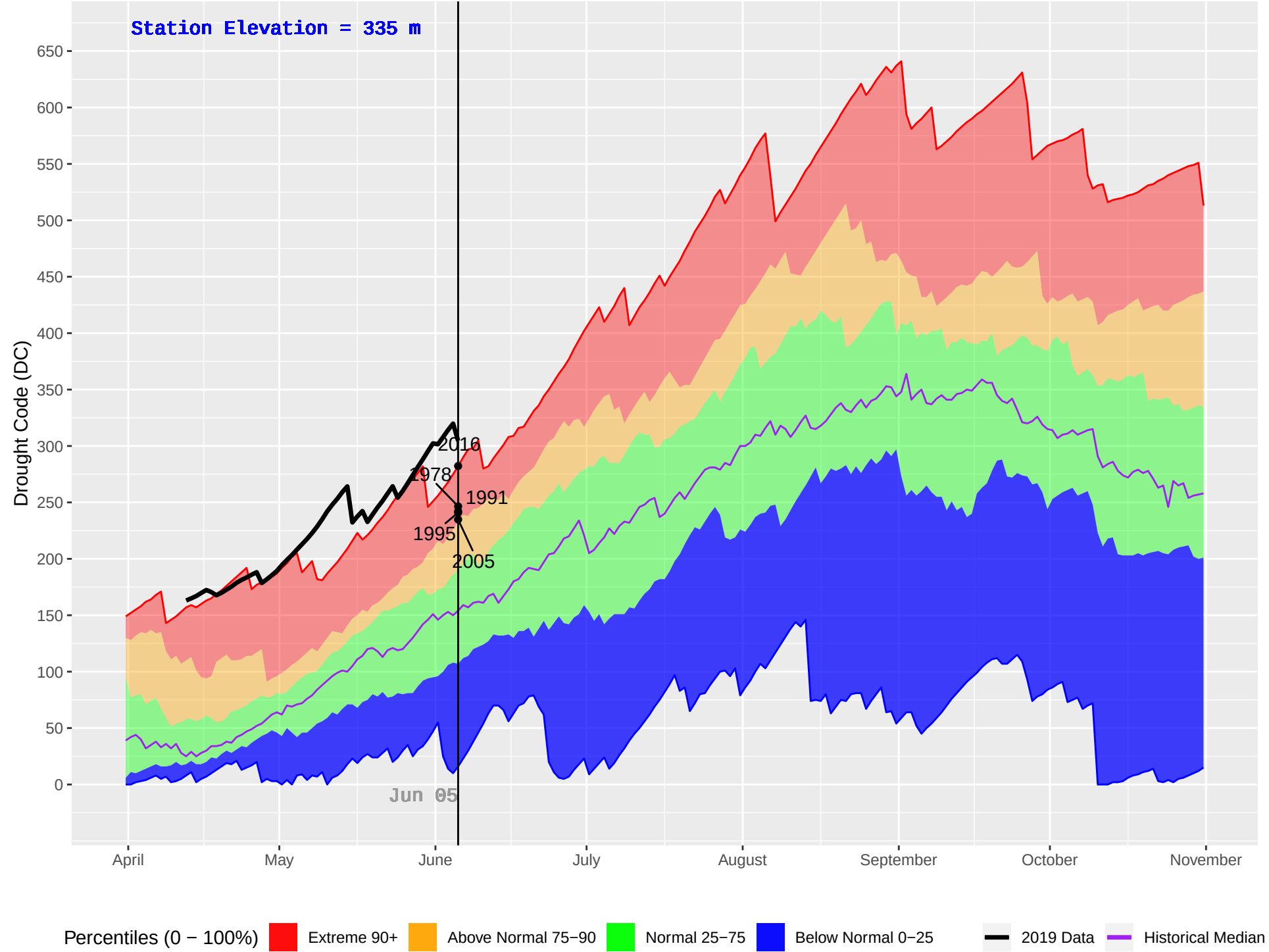
KISPIOX HUB (428) : Historical (1970–2018) and Current (2019) Daily Drought Code (DC)
