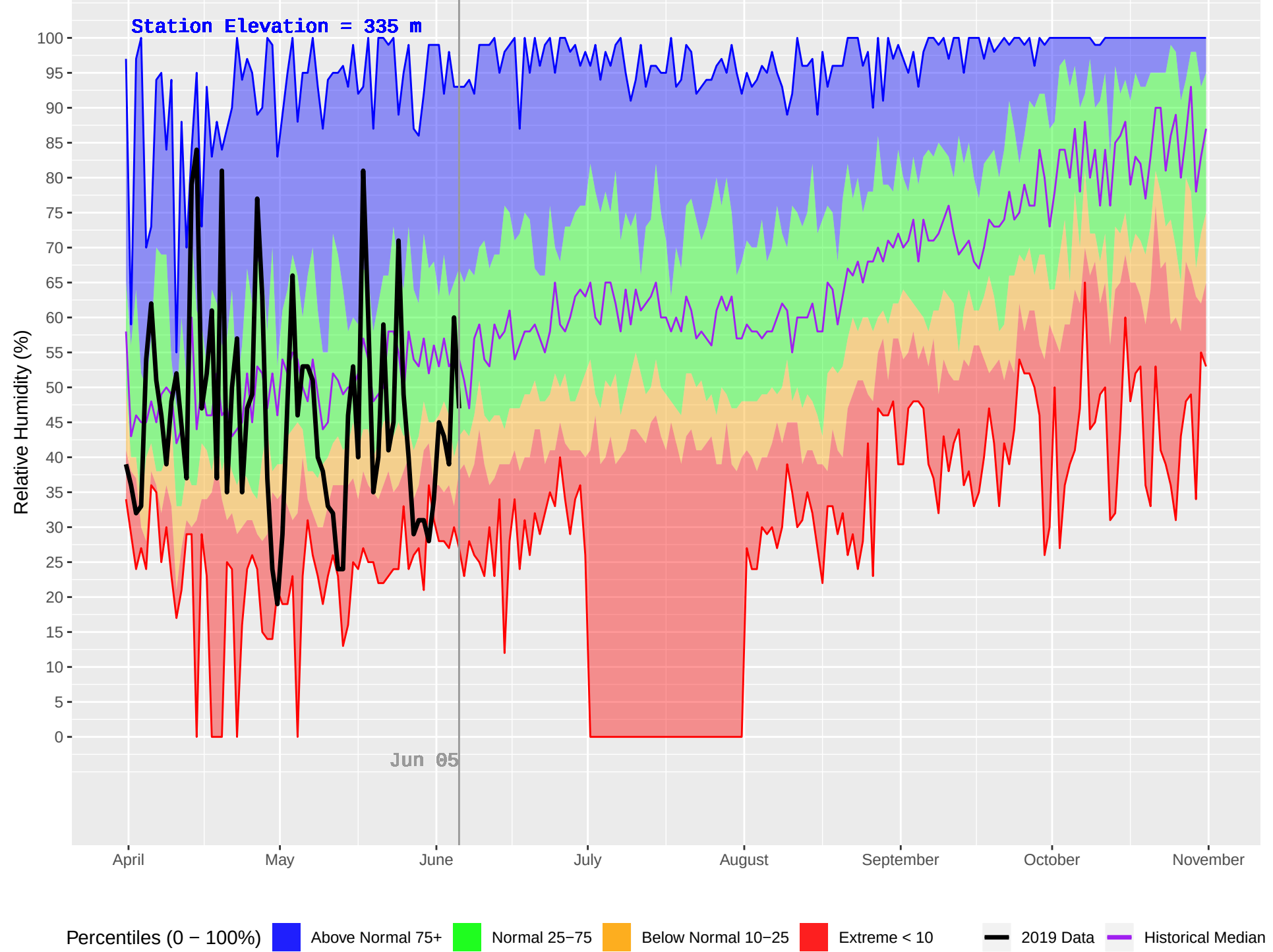
KISPIOX HUB (428) : Historical (1970–2018) and Current (2019) Daily Relative Humidity
