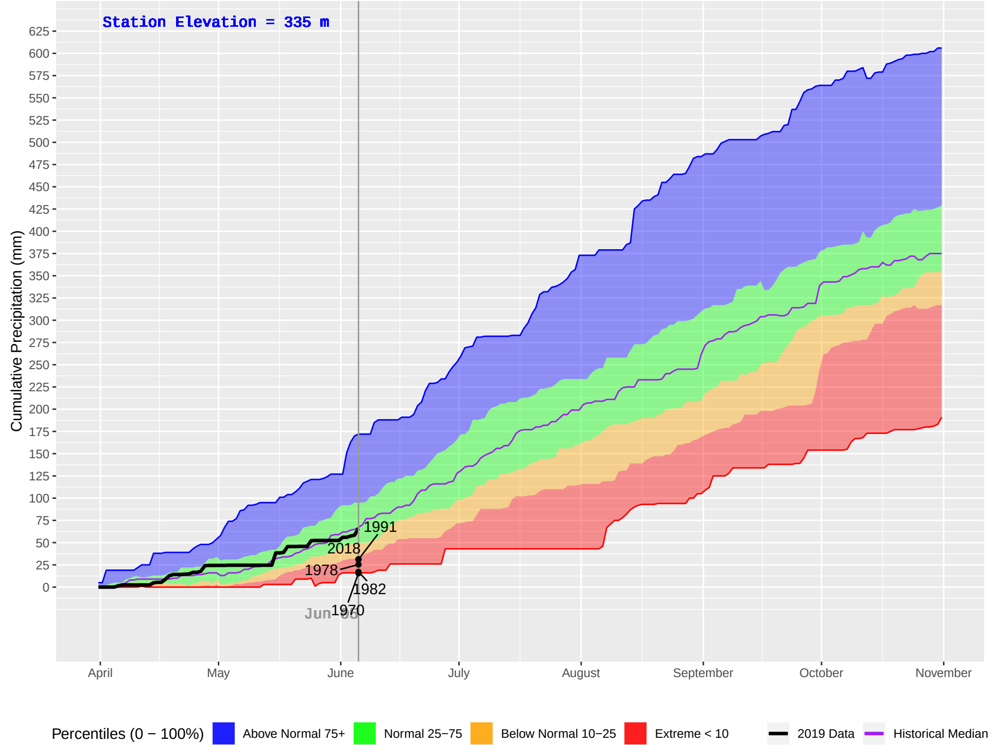
KISPIOX HUB (428) : Historical (1970–2018), Current (2019) Daily Cumulative Precipitation
