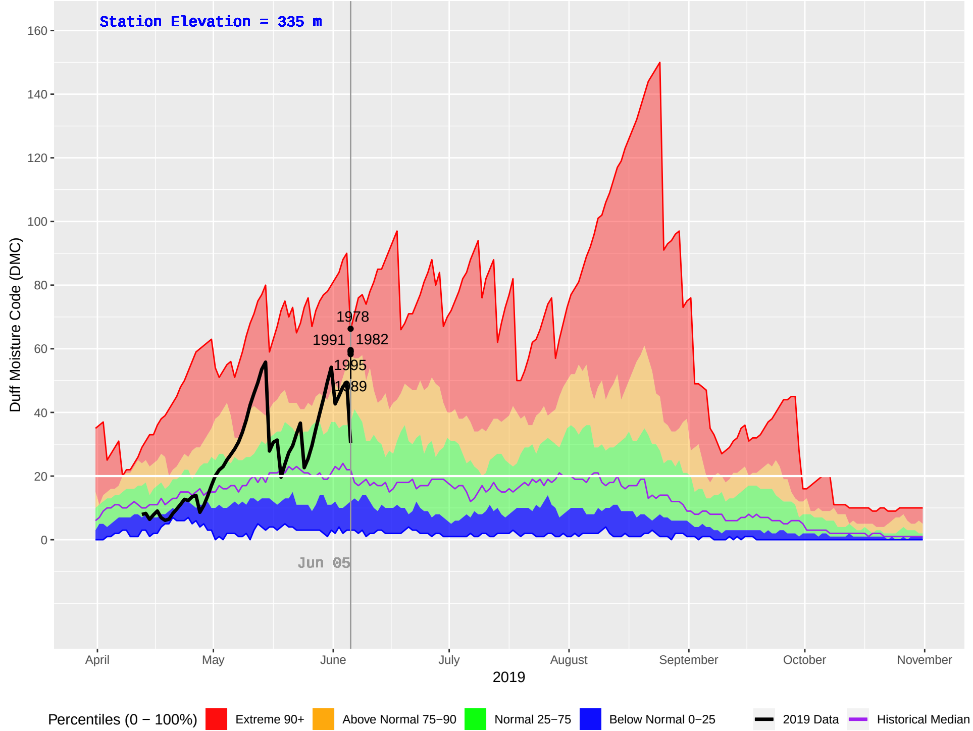
KISPIOX HUB (428) : Historical (1970–2018), Current (2019) Daily Duff Moisture Code (DMC)
